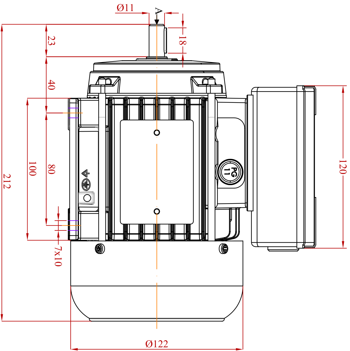
VIEW-A
