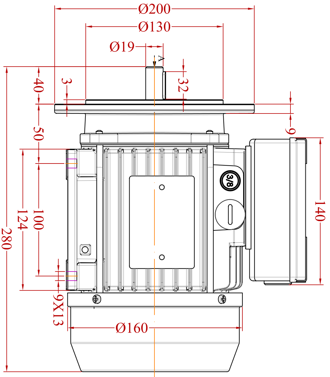
VIEW-A
