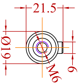
VIEW-A
